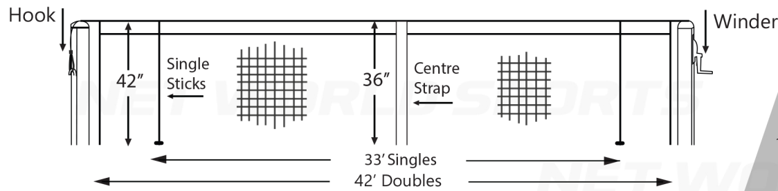
Fig 9: Tennis Net Dimensions
