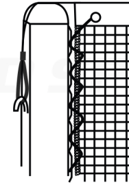
Fig 7: Fixed Lacing Bar
