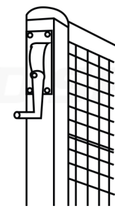
Fig 2: Internal Winder
